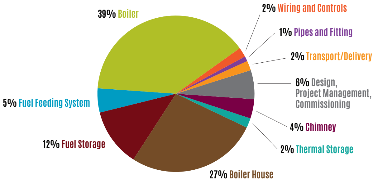
FIGURE 17: Example of capital cost breakdown where a new boiler house is required Based on BERCC analysis of project costs
